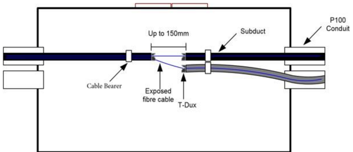
Proposed Multi Subduct Interchange Design – Side View
