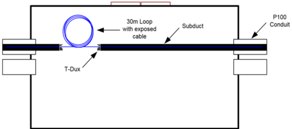
Existing Loop Design – Side View
