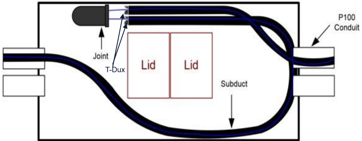
Existing Joint Design – Top View
